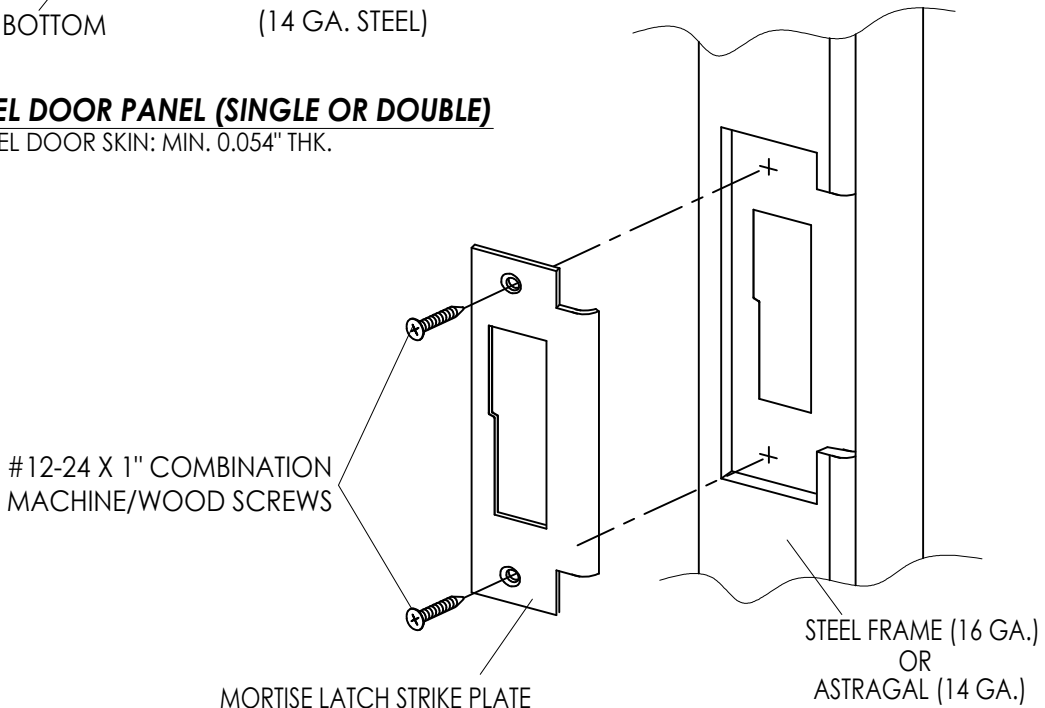
STRIKE PLATE DETAILS
